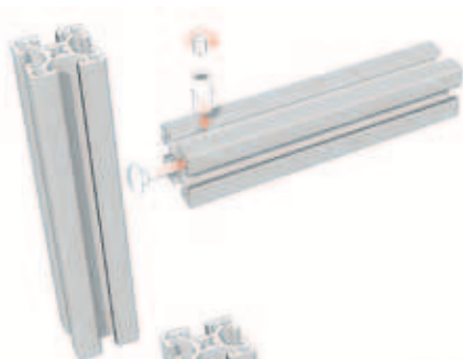
Conector Perpendicular
