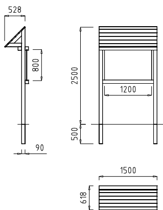
MI007 - MI008 E: 1/100
