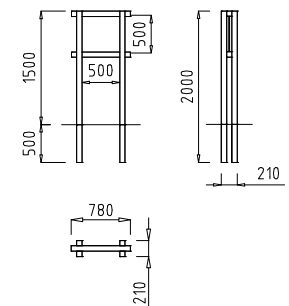
MI005 - MI006 - MI012 E: 1/100
